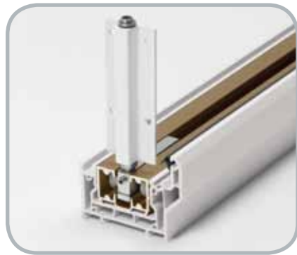
In-built rollers
